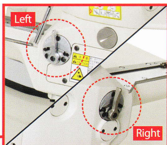
Differential feed ratio adjustment levers
