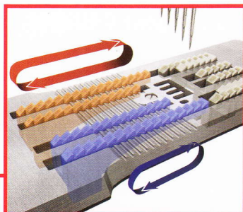
Right and left independent differential feed adjustment mechanism
