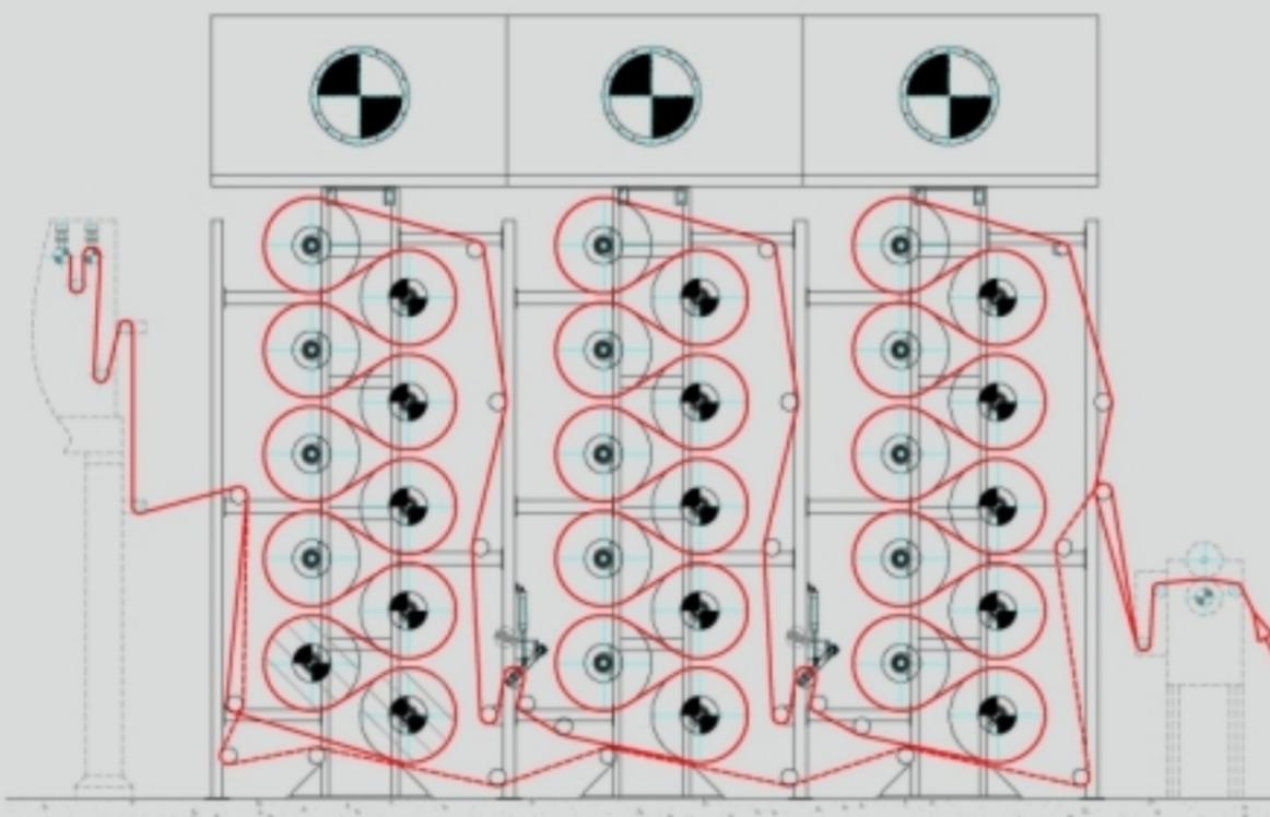
DRYING UNIT (DENIM) FABRIC PROCESSING
