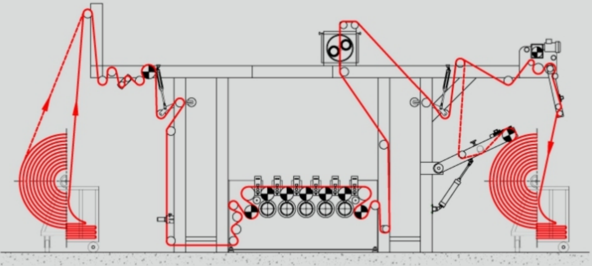
SUEDING & EMERIZING FABRIC PROCESSING
