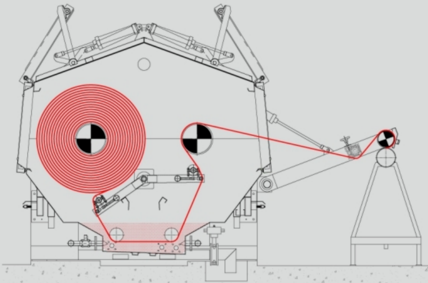
ATMOSPHERIC JIGGER FABRIC PROCESSING
