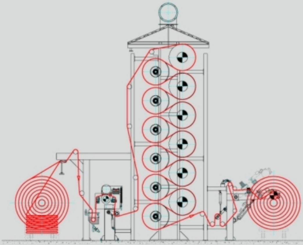
DRYING UNIT WIT SQUEEZING FLOULARD FABRIC PROCESSING
