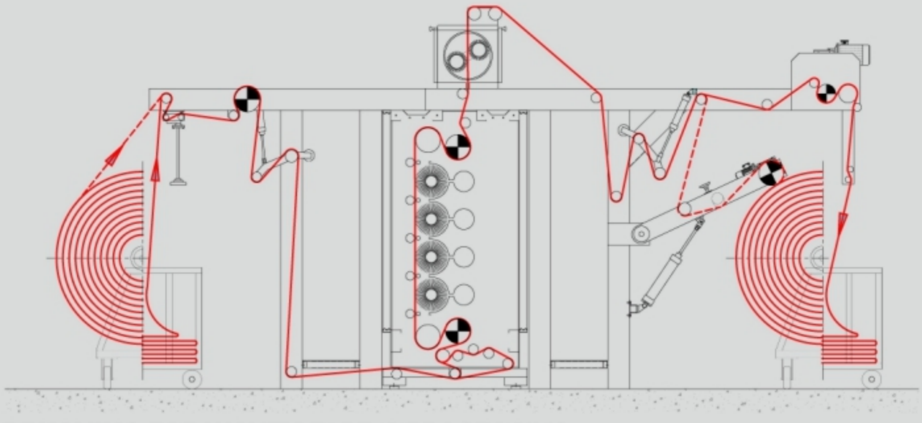
BRUSHING FOR WOVEN FABRIC PROCESSING
