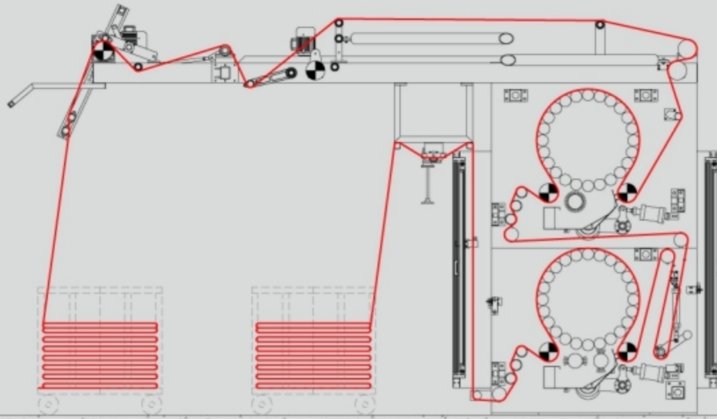
RAISING FABRIC PROCESSING
