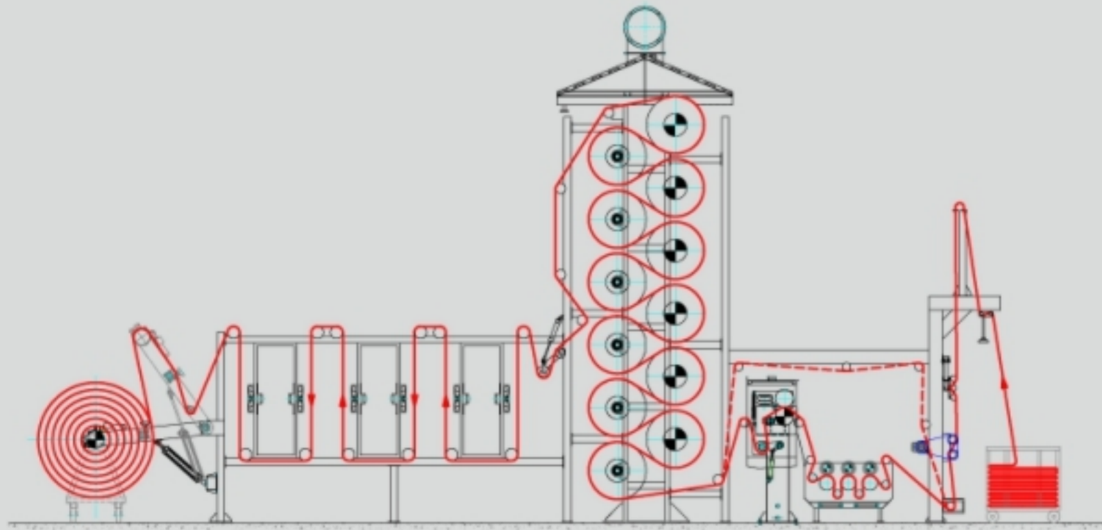
DRYING UNIT (VELVET) FABRIC PROCESSING
