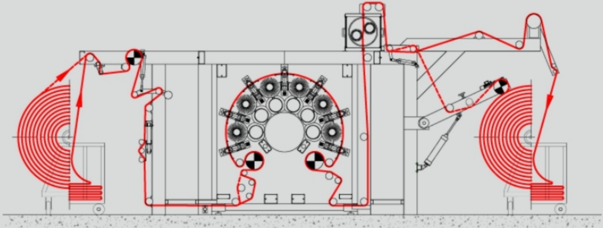
BRUSHING FOR WOVEN & KNITTED FABRIC PROCESSING
