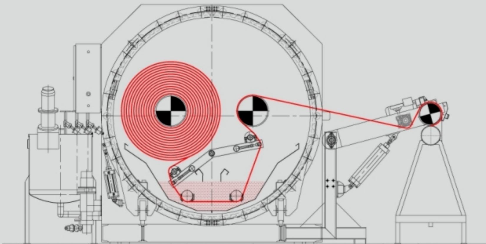
HIGH TEMPRATURE JIGGER FABRIC PROCESSING
