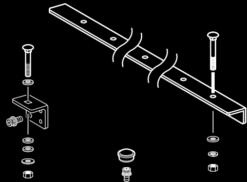
Semi-submerged set
